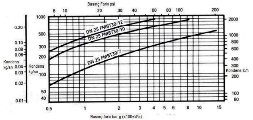
DN25 FMBT30
